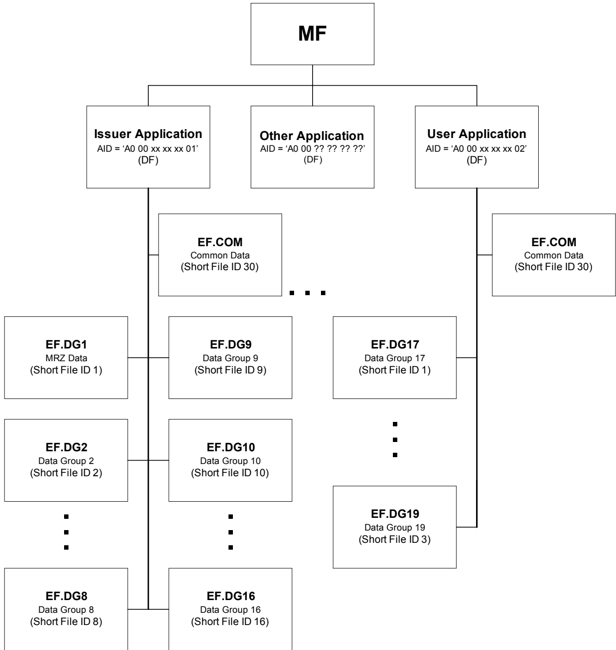
Figure X1 – IC Card File Structure
